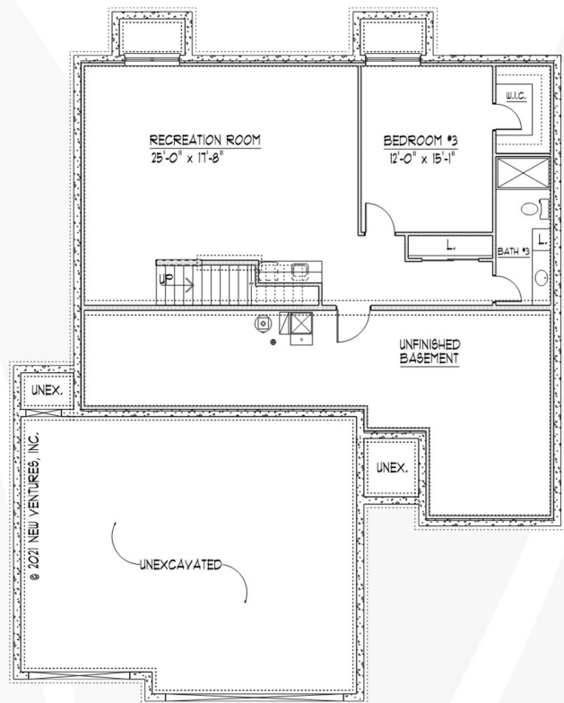
BASEMENT LEVEL FLOOR PLAN (922 SF FINISHED BASEMENT)
